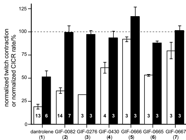
Figure 1. Effects of dantrolene ( 1 ) (20 μM) and its derivatives 2–7 (50 μM) on twitch contraction (open column) and CICR (filled column) of mouse skeletal muscle. The magnitude of twitch contraction and the rates of Ca 2+ release in the presence of 1 or its derivatives were normalized to the control value (100%) obtained in the absence of these compounds. The data for compounds 1–3 are cited from Ref. 9a. The numbers of experiments ( n ) are indicated in the column.
