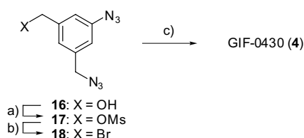
Scheme 3. Synthesis of GIF-0430 ( 4 ). Reagents and conditions: (a) MsCl, Et 3 N, CH 2 Cl 2 , 0 °C, 3.5 h, 94%; (b) KBr, DMF, rt, 13 h, 99%; (c) 1 , DMF, rt, 22 h, 79%.
