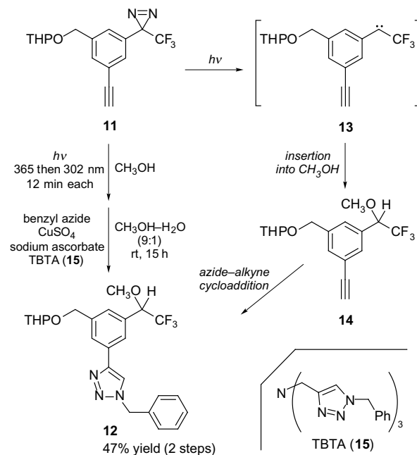
Scheme 2. Photoreaction of ethynyl-functionalized phenyltrifluoromethyldiazirine 11 in methanol followed by cycloaddition with benzyl azide (THP = tetrahydropyran-2-yl).
