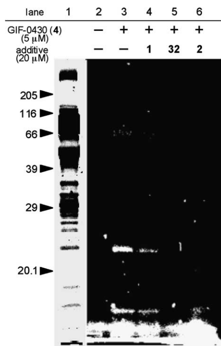
Figure 2. SDS-PAGE analysis of rabbit TC fraction (1.0 mg/mL, 20 µg total proteins) photolabeled with 5 µM of GIF-0430 ( 4 ) in the absence or presence of dantrolene ( 1 ), its derivative, GIF-0162 ( 32 ) or GIF-0082 ( 2 ) (20 µM), followed by Staudinger–Bertozzi ligation with GIF-0373 ( 33 ) (500 µM) overnight. The photograph was taken with a monochrome CCD camera (ATTO, Printgraph AE-6914) and visualized on a UV transilluminator (UVP, TLW-20, 365 nm, 8 W × 4). For comparison, Coomassie brilliant blue (CBB)-stained proteins contained in the TC fraction are shown in lane 1. The arrowheads and the attached numbers ( M_r \times 10^3 ) indicate apparent values of the fluorescent high molecular weight marker (Sigma).
