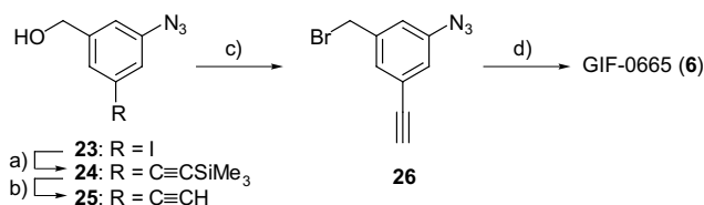
Scheme 5. Synthesis of GIF-0665 ( 6 ). Reagents and conditions: (a) Me 3 SiC≡CH, Pd 2 (dba) 3 , ( n -Bu) 4 NOAc, DMF, rt, 0.5 h, 64%; (b) KOH, MeOH, 0 °C to rt, 0.5 h, 88%; (c) CBr 4 , PPh 3 , CH 2 Cl 2 , rt, 0.5 h, 88%; (d) 1 , DMF, 0 °C to rt, 2 h, 61%.
