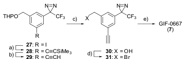
Scheme 6. Synthesis of GIF-0667 ( 7 ). Reagents and conditions: (a) Me 3 SiC≡CH, (Ph 3 P) 2 PdCl 2 , CuI, Et 3 NH, rt, 13 h, 77%; (b) KOH, MeOH, 0 °C to rt, 0.5 h, 91%; (c) pyridinium p -toluenesulfonate, EtOH, 50 °C, 19 h, 98%; (d) CBr 4 , PPh 3 , CH 2 Cl 2 , rt, 2.5 h, 82%; (e) 1 , DMF, 0 °C to rt, 2 h, 85%.
