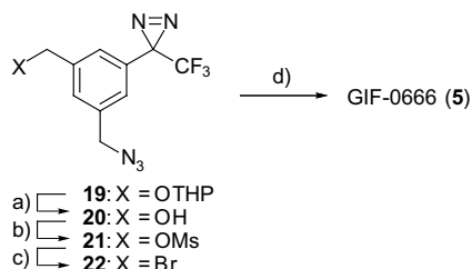
Scheme 4. Synthesis of GIF-0666 ( 5 ). Reagents and conditions: (a) pyridinium p -toluenesulfonate, EtOH, 55 °C, 12 h, 94%; (b) MsCl, Et 3 N, CH 2 Cl 2 , 0 °C, 1.5 h, 99%; (c) KBr, DMF, 0 °C to rt, 13 h, 95%; (d) 1 , DMF, rt, 17 h, 78%.
